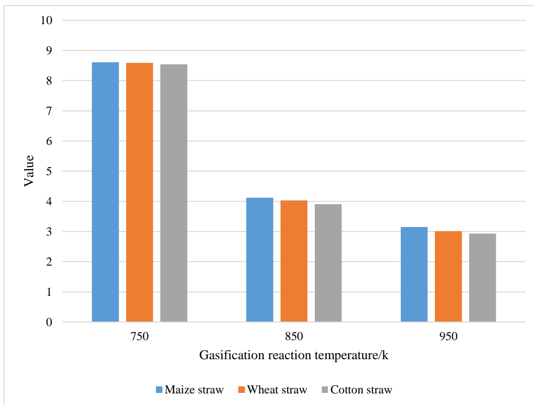
Figure 2. Characteristics of the carbamemolar ratio of the three samples varying with the reaction temperature
