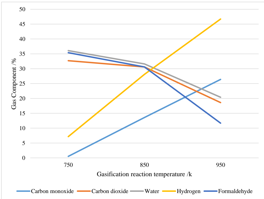
Figure 1. Characteristics of cotton straw syngas components changing with the reaction temperature
