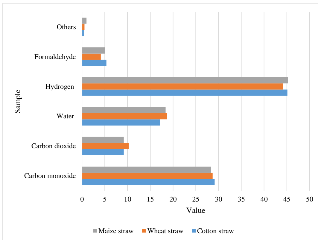
Figure 3. Syngas components generated from balanced solar-biomass gasification
