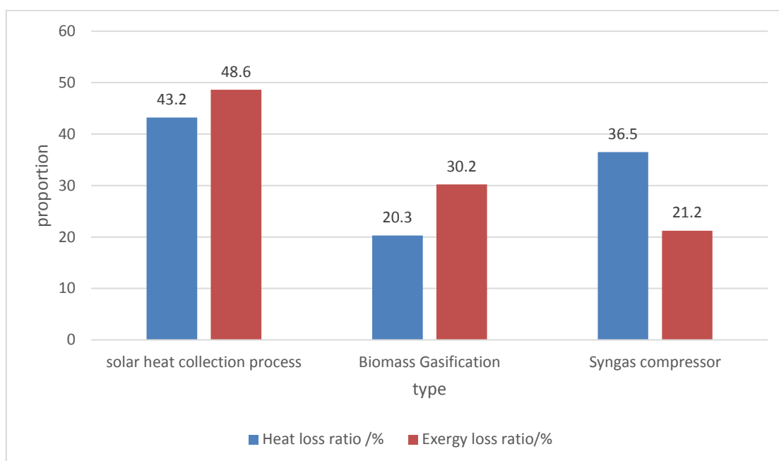
Figure 3. System heat balance and exergy balance analysis diagram
