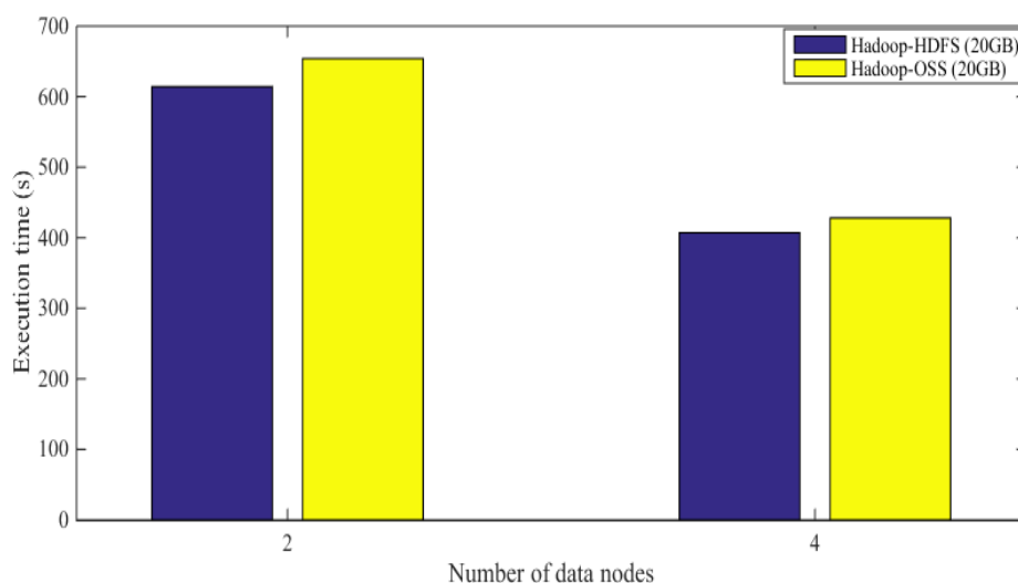
Figure 1. WordCount experiment results after modifying the file block size
