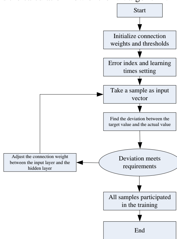
Figure 2. NN algorithm process
