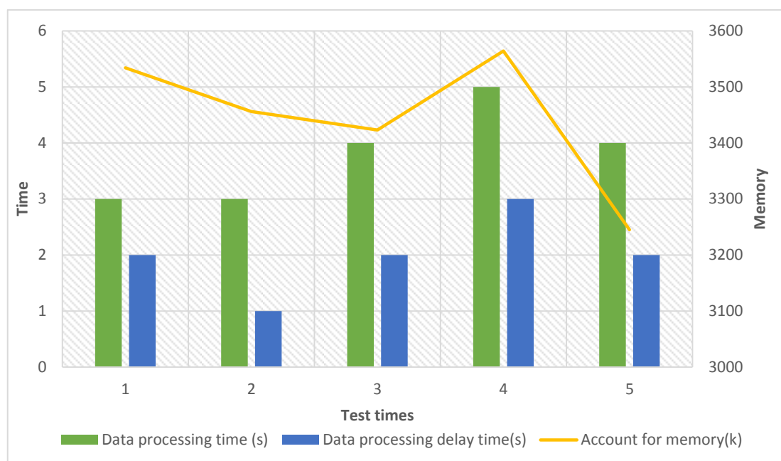
Figure 4. Performance test of the marine resource growth model
