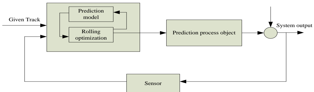
Figure 2. Coordinated prediction model control
