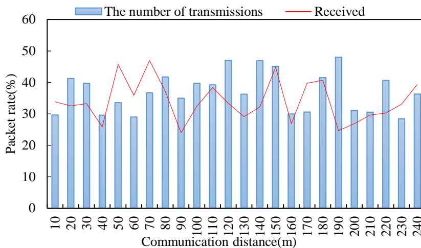
Figure 8. Testing the communication distance of the wireless sensor network
