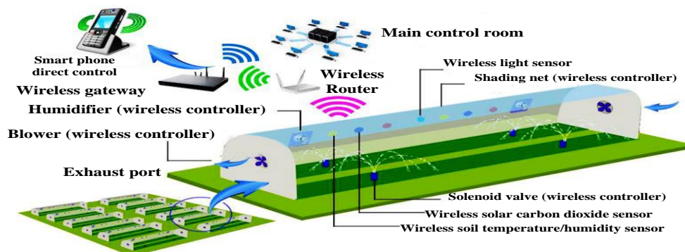
Figure 1. Smart agricultural greenhouse
