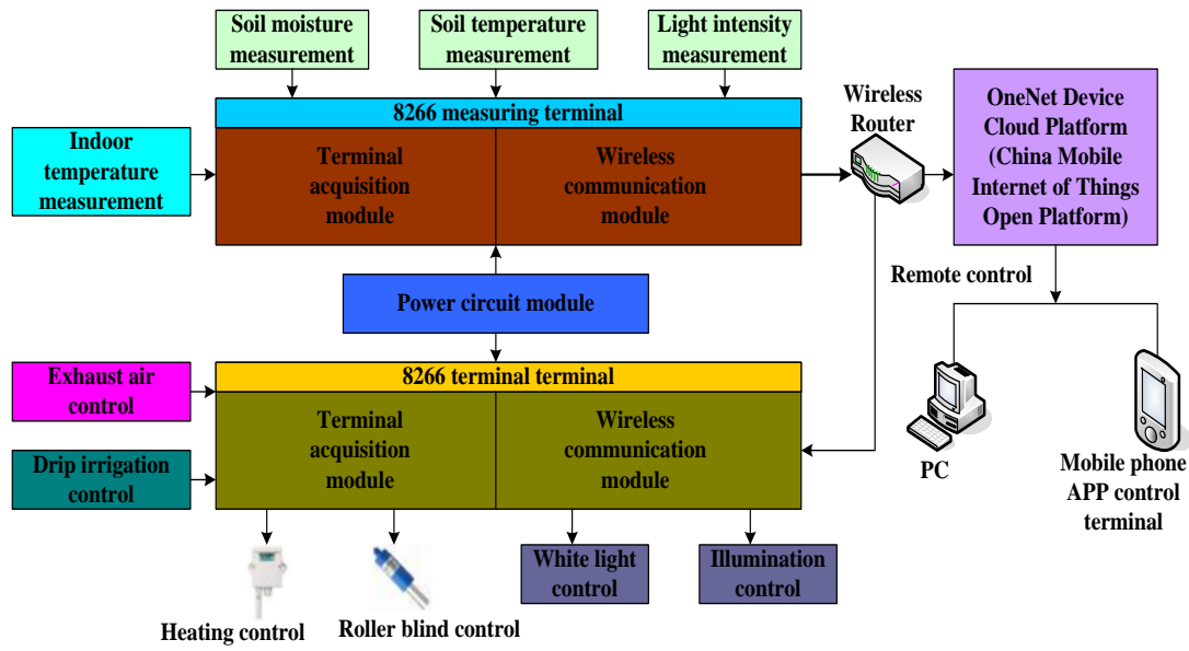
Figure 3. The overall design scheme of the remote monitoring system for the intelligent agricultural greenhouse based on the cloud platform
