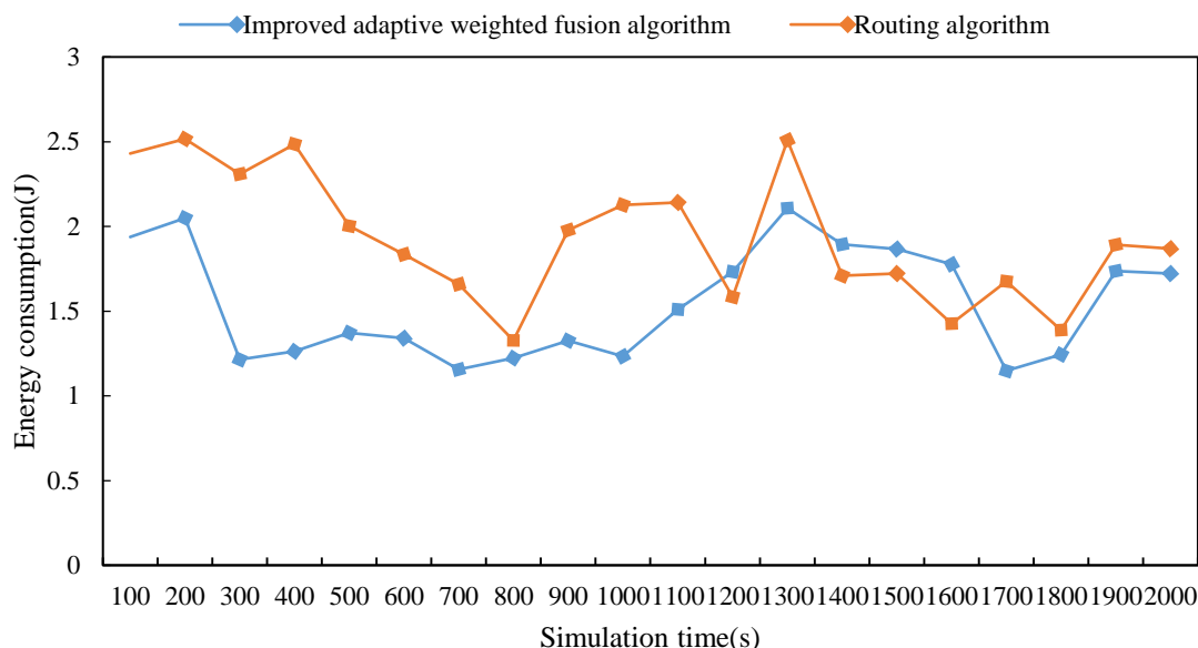
Figure 6. Energy consumption of cluster head nodes by comparing improved adaptive weighted fusion algorithm and routing algorithm
