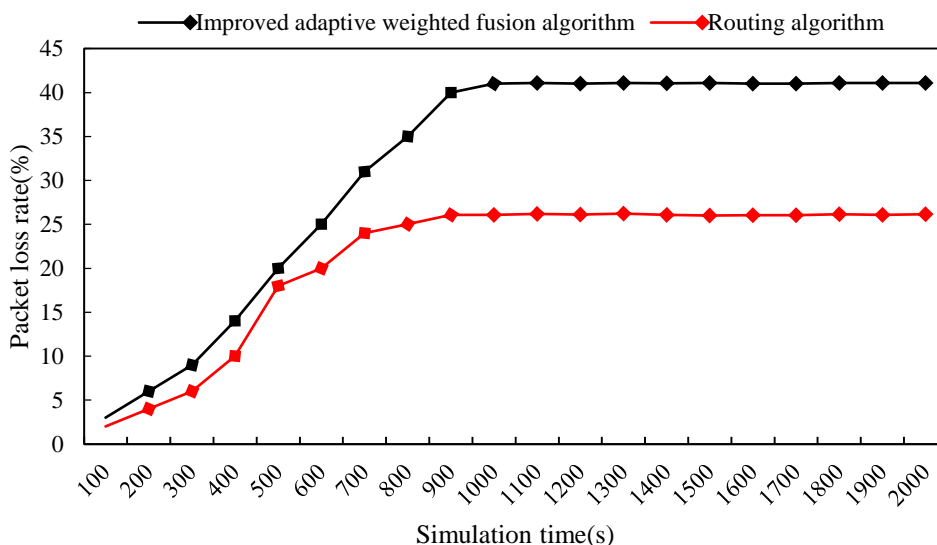
Figure 7. The packet loss rate of the improved adaptive weighted fusion algorithm and routing algorithm
