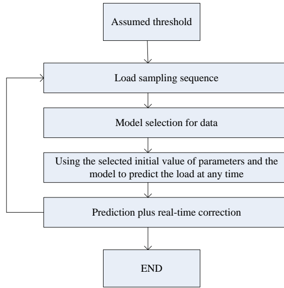
Figure 2. Linear time-series model
