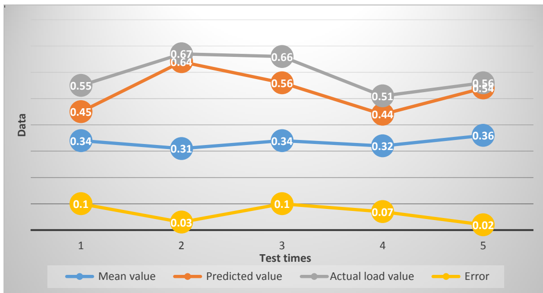
Figure 4. Predicted value
