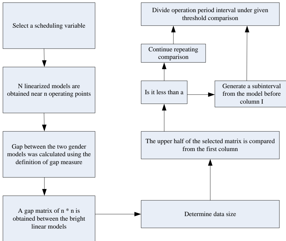
Figure 3. Distributed system host load prediction model
